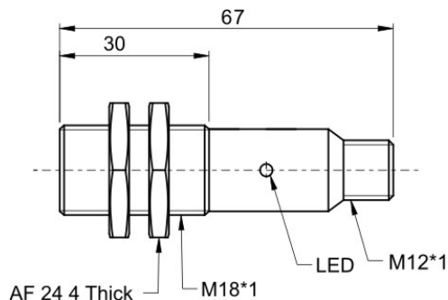
Dimension drawing
