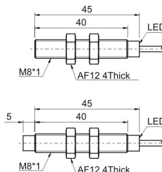
Dimension drawing
